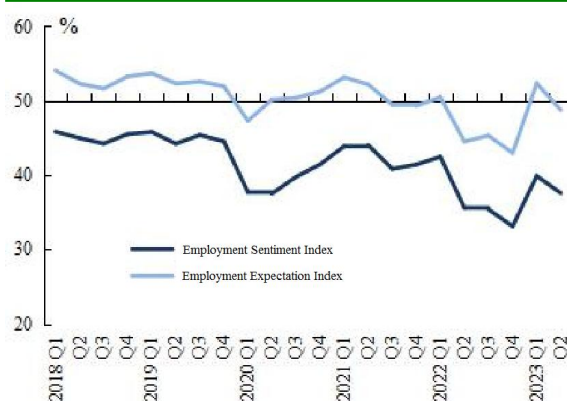
Figure 2: Employment Sentiment Index and Employment Expectation Index
